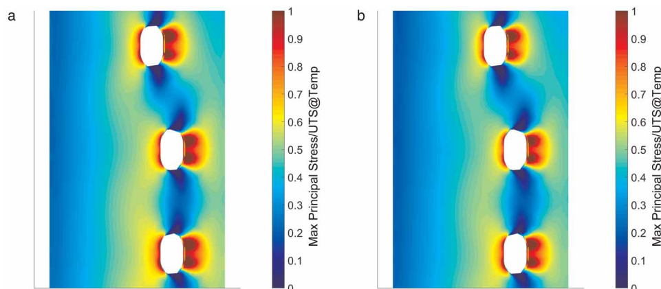
Figure 12. Combined HTC adjustments - stress distribution: (a) thermal FEA, (b) combined adjustments.
