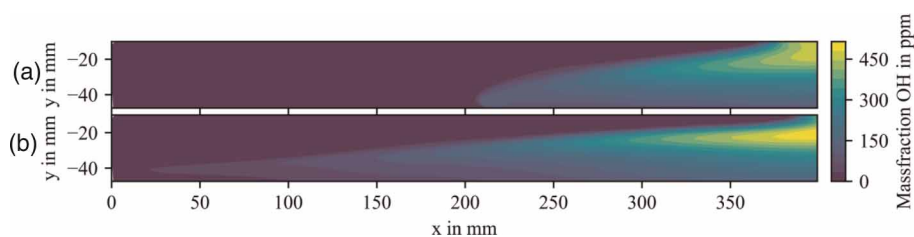
Figure 11. Comparison for the OH-radical distribution for (a) simulation without and (b) simulation with CHT. The data is shown for y < 0 mm and x < 400 mm.
