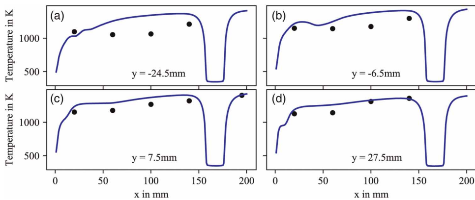
Figure 5. Comparison between thermographic phosphor measurements (circles) and CHT simulation (line) of the combustion chamber inner wall temperature at constant values of y .
