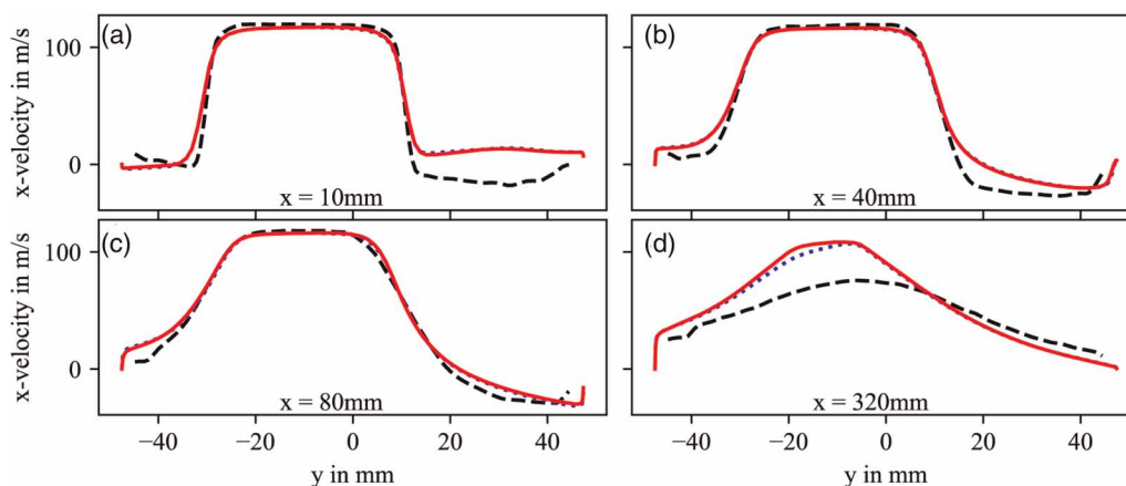
Figure 7. Comparison between PIV measurement (black dashed line) and simulations with (solid red line) and without (dotted blue line) CHT for constant values of x .
