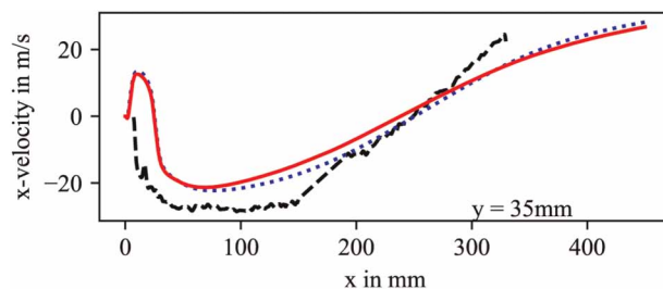
Figure 8. Comparison between (PIV measurement (black dashed line) and simulations with (solid red line) and without (dotted blue line) CHT for constant values of y .
