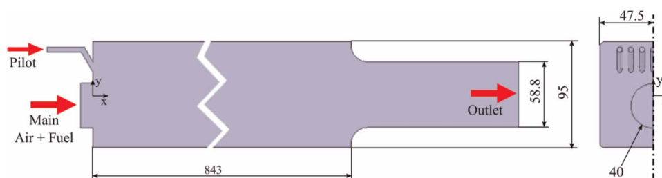
Figure 1. Schematic of the FLOX model combustion chamber with coordinate system and dimensions (mixing-duct and injector geometry are not shown).
