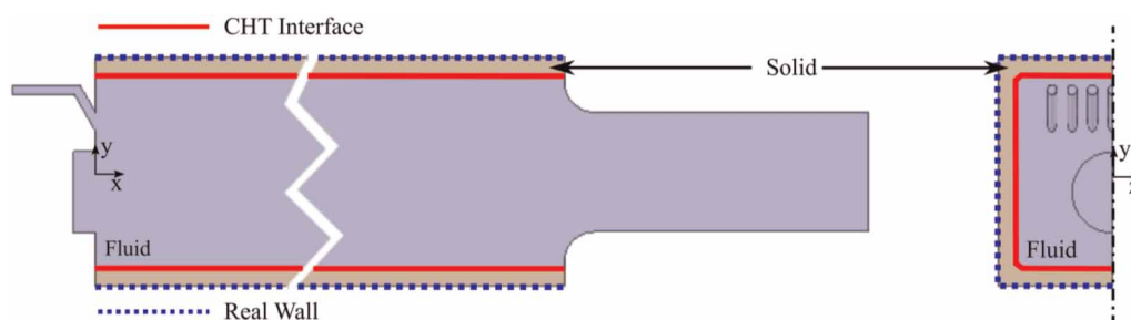
Figure 2. Computational domain for fluid and solid.
