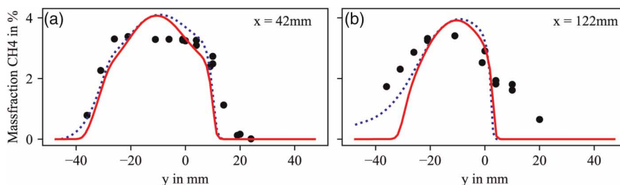
Figure 9. Radial species profiles for \text{CH}_4 at different locations for constant values of x . The circles correspond to the measurement points while the red solid the represents the simulation with CHT and the blue dashed line represents the simulations without CHT.
