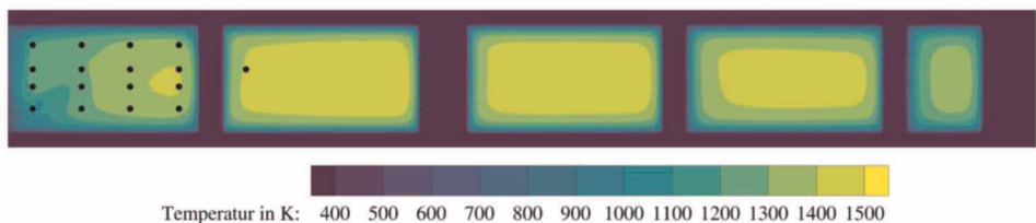
Figure 3. Wall temperature of the combustion chamber resulting from the simulation with CHT. Circles represent available measurement points.
