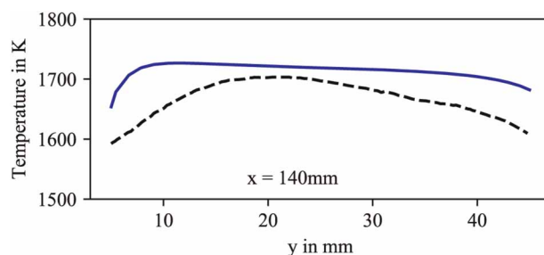
Figure 6. Comparison between temperature measurements derived from OH-LIF measurements (dashed black line) and CHT simulation (blue solid line) of the combustion chamber inside fluid temperature for x = 140 mm.
