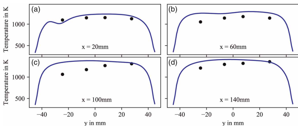
Figure 4. Comparison between thermographic phosphor measurements (circles) and CHT simulation (line) of the combustion chamber inner wall temperature at constant values of x .
