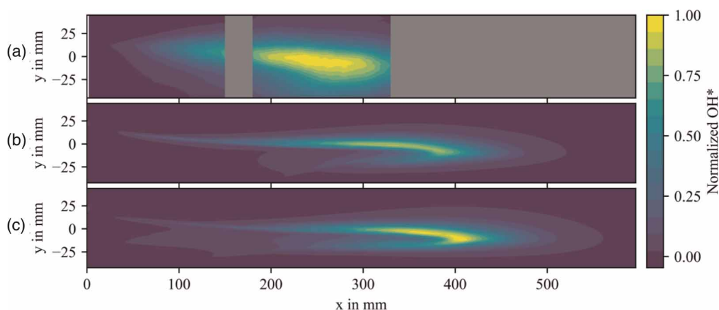
Figure 10. Comparison between OH*-CL measurement (a) and simulations without (b) and with (c) CHT. Absolute values for each contour plot are normalized by the individual maximum value. Greyed regions represent areas with no data available.
